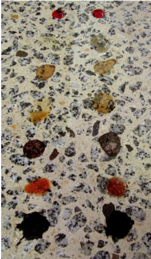
←→ ←→ Concrete treated with HiperGuard Premium - Enhance. Untreated.
